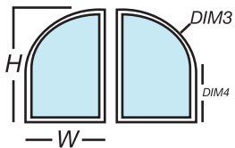
QXL or QXR Quarter Arch (L or R) with Extended Legs Required Dim: W, H, DIM4 Width and radius are equal. View required for single units: OSLI or ISLO
