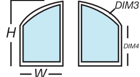
EXL or HXR* Half Eyebrow (L or R) with Extended Legs Required Dim: W, H, DIM4 DIM4 must be above profile limits. View required for single units: OSLI or ISLO
