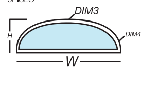
EP Ellipse Required Dim: W, H DIM4 (Minor Radius) must be above profile limits.
