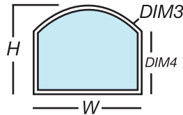
EBX Eyebrow with Extended Legs Required Dim: W, H, DIM4 Height of curve must be less than height of half the width. DIM4 must be above profile limits.
