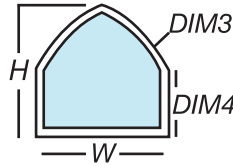
CHX Cathedral with Extended Legs Required Dim: W, H, DIM4 DIM3 (Radius) must be above profile limits.
