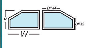
PTL or PTR Pentagon (L or R) Required Dim: W, H, DIM3, DIM4 View required for single units: OSLI or ISLO
