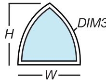
CH Cathedral Required Dim: W, H DIM3 (Radius) must be above profile limits.
