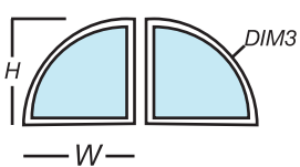
QAL or QAR* Quarter Arch (L or R) Required Dim: W, H On Quarter Arches, the width and height are equal. View required for single units: OSLI or ISLO
