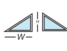
TRL or TRR Triangle (L or R) Required Dim: W, H View required for single units: OSLI or ISLO
