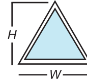
TRE Triangle Equilateral Required Dim: H On this style, all sides are equal.
